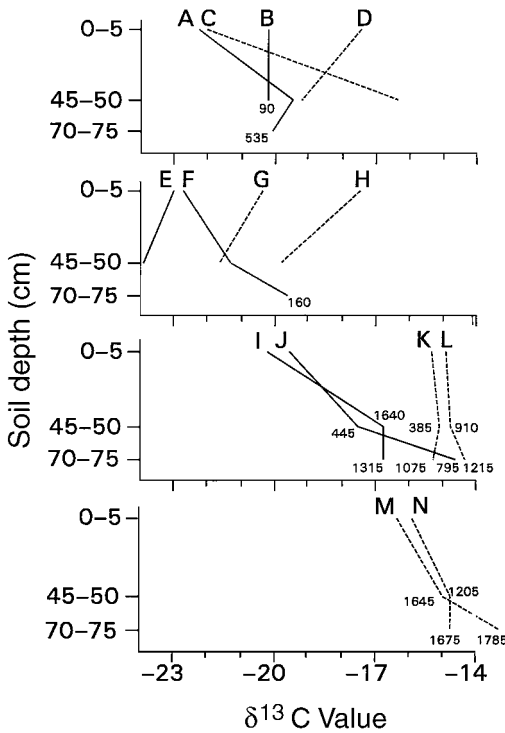
Figure 4.4 Stable carbon isotopic composition and ^{14}\text{C} dates for soil organic matter at different soil depths along a transect through a Quercus savanna into a \text{C}_4 semi-desert grassland in southern Arizona, United States. Each line represents a single soil core. Soil cores A-D are 500 m above the savanna-grassland ecotone, cores E-H are 150 m above the ecotone, I-L are at the savanna-grassland ecotone, and cores M and N are 150 m below the ecotone in the grassland. Solid lines are cores collected beneath trees and dashed lines are cores collected beneath grasses >5 m from a tree canopy. Values adjacent to lines are ^{14}\text{C} dates (in years) at different depths; all depths without dates had postmodern signatures. Reproduced with permission from McClaran and McPherson (1995).
